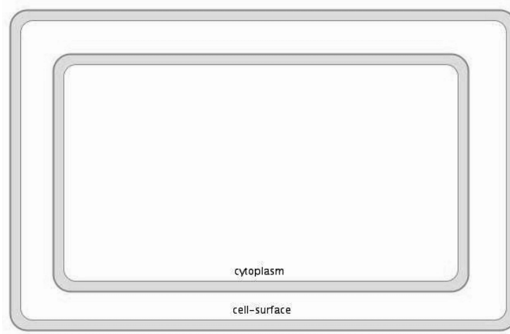
Fig. 2. Graphical representation of the membrane structure specifying an E. coli bacterium.
